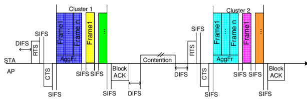
Fig. 2. Contention and transmission procedure in one4all scheme
